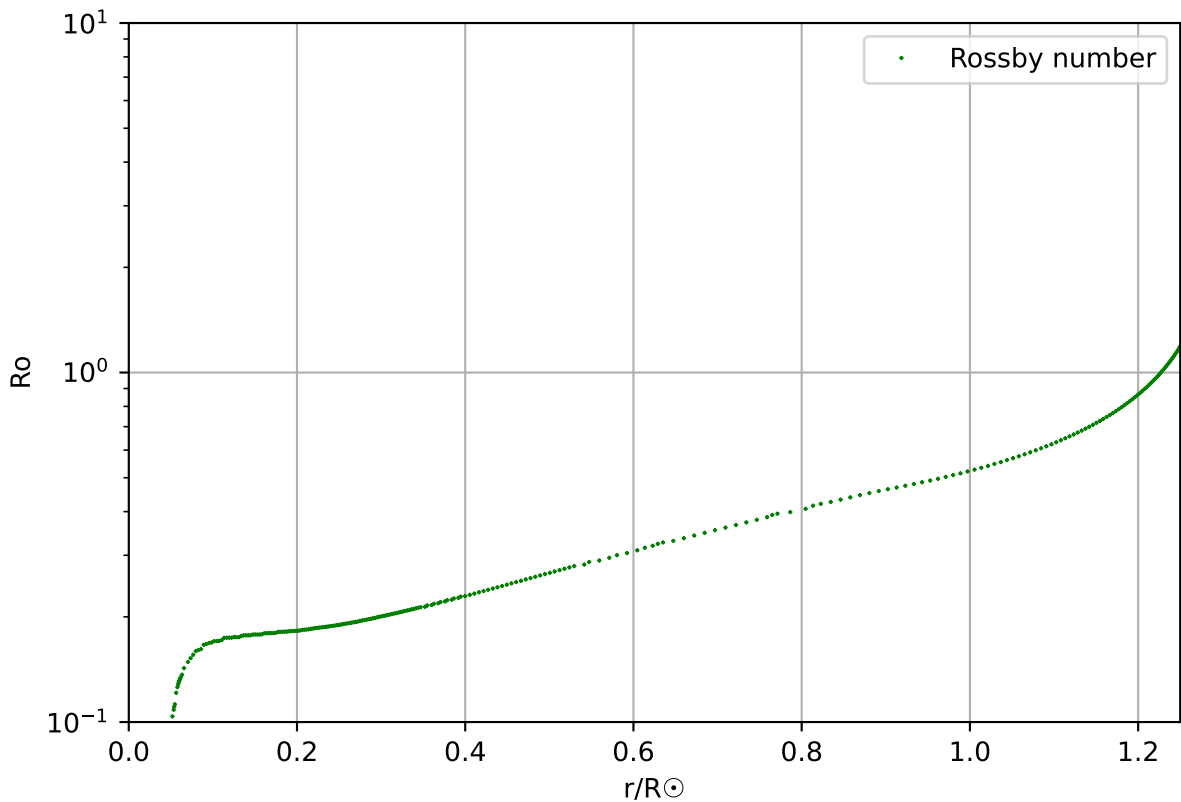
Rossby number, profile 170, age 9.94 \times 10^9
